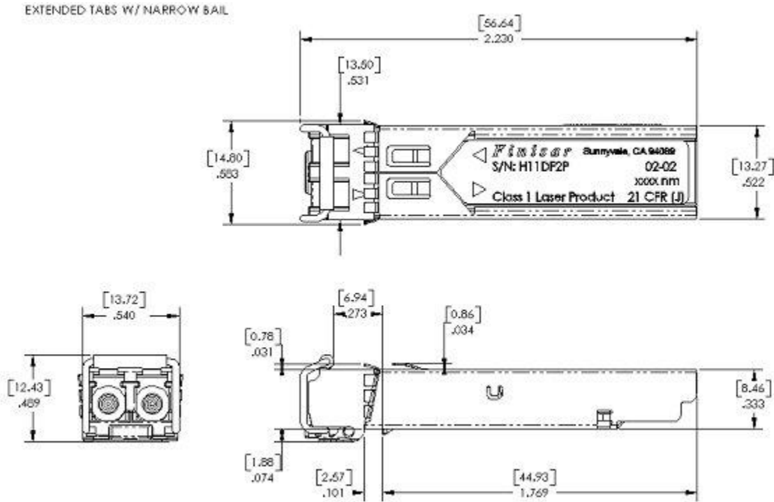
FWLFI621P2Txx Outline Drawing - units in inches [mm]
